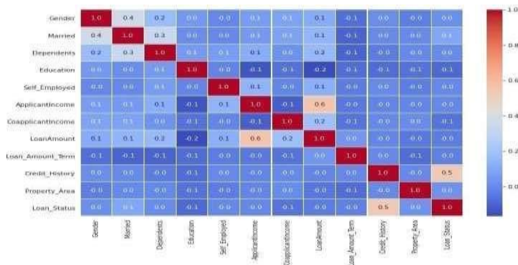
Figure 2: The correlation among all the attributes in the dataset
